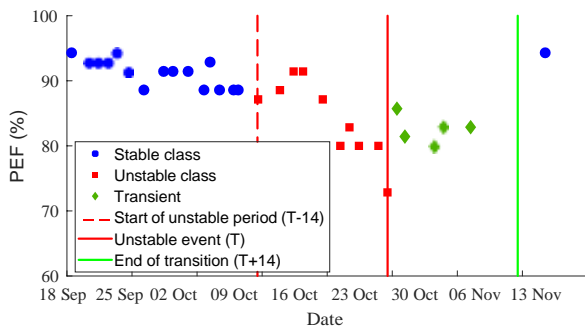
Fig. 2. Data class label surrounding unstable event
